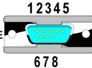
Making the RJ45 to RS422 male adapters
