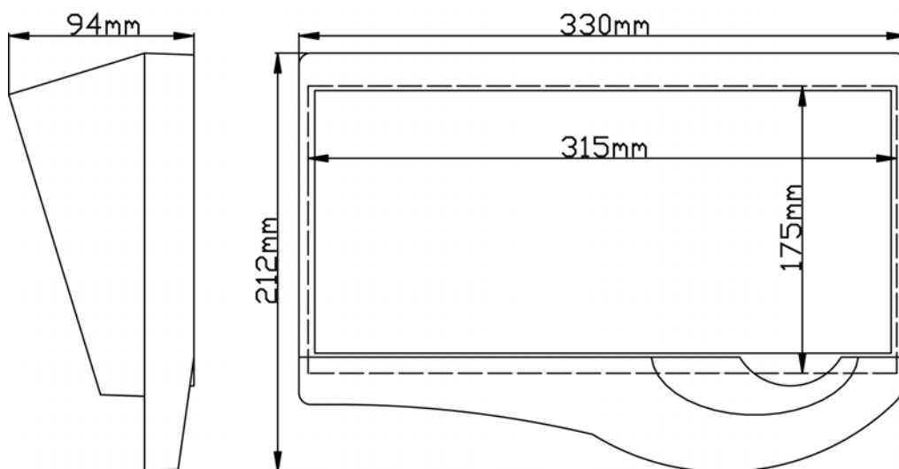
HT88x/c/s Outline dimensions
