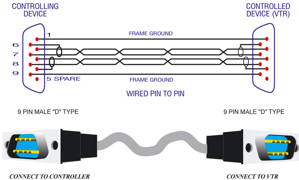
Standard RS422 cable
