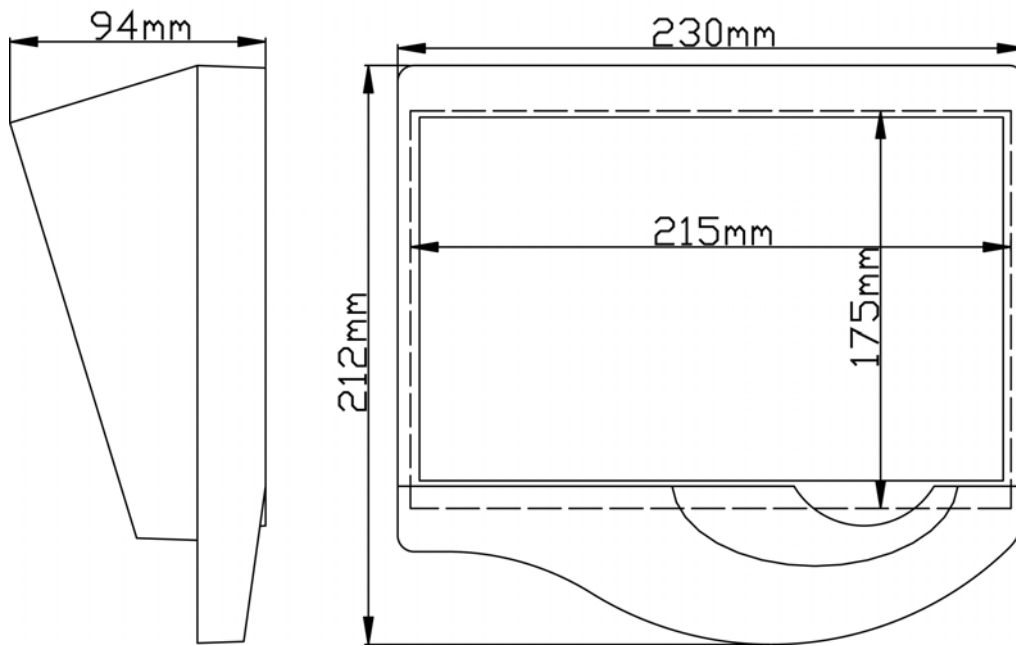
HT88x Outline dimensions
