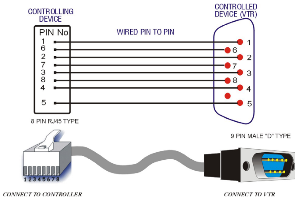
RJ45 to D type - RS422 cable
